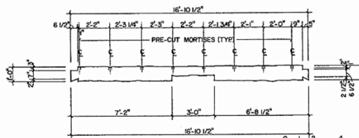
LOG DETAIL
